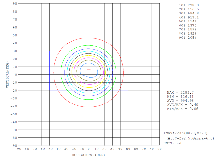
Isocandela Diagram
